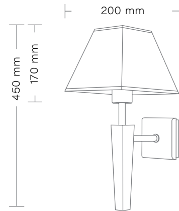
TOPAZ Kinkiet/Wall lamp max 1 x 40W, Gwint/Chip: E27 Zasilanie/Power: 230V
