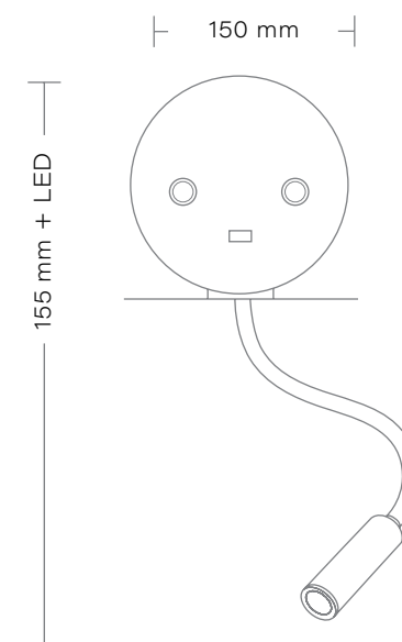
NEVADA K-4 Kinkiet/Wall lamp 1 x 3W LED + 6W LED Zasilanie/Power: 230V USB
