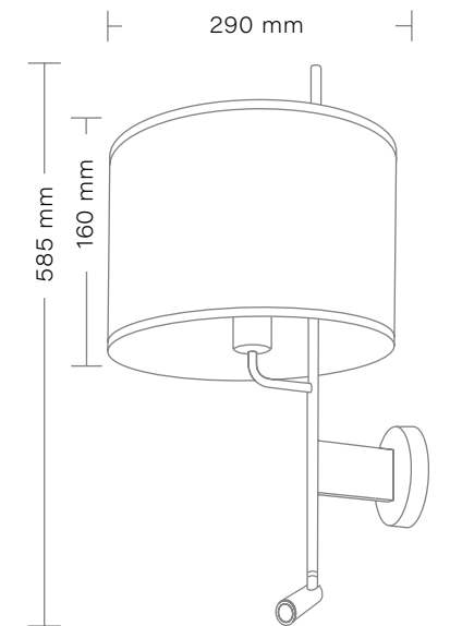
PORTO K-2 LED Kinkiet/Wall lamp max 1 x 40W, 1 x 3W LED Gwint/Chip: E27 Zasilanie/Power: 230V
