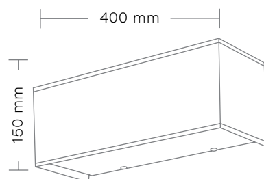
VIENNA K-2 Kinkiet/Wall lamp max 2 x 40W Gwint/Chip: E27 Zasilanie/Power: 230V
