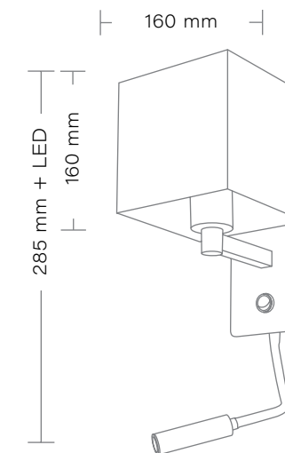
FOBOS Kinkiet LED/ Wall lamp LED max 1 x 40W 1 x 3W LED Gwint/Chip: E27 Zasilanie/Power: 230V
