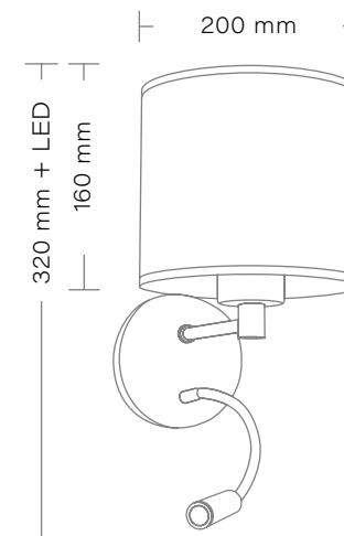
DOS Kinkiet LED / 330 Wall lamp LED / 330 max 1 x 40W 1 x 3W LED Gwint/Chip: E27 Zasilanie/Power: 230V
