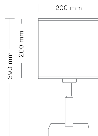
QUATTRO Lampa gabinetowa/ Big table lamp max 1 x 40W Gwint/Chip: E27 Zasilanie/Power: 230V
