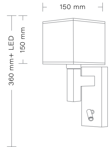
QUATTRO Kinkiet LED / 90 Wall lamp LED / 90 max 1 x 40W, 1 x 3W LED Gwint/Chip: E27 Zasilanie/Power: 230V
