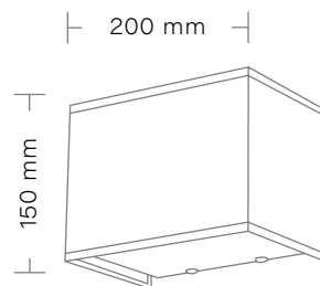
VIENNA K-1 Kinkiet/Wall lamp max 1 x 40W Gwint/Chip: E27 Zasilanie/Power: 230V
