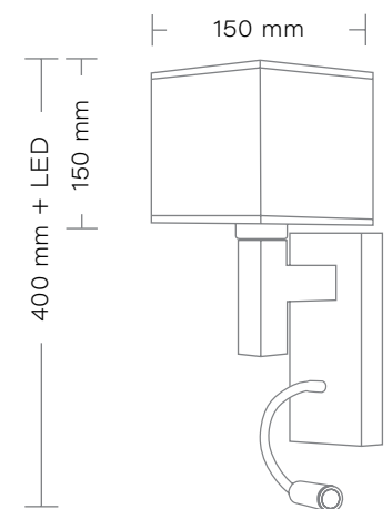
QUATTRO Kinkiet LED / 330 Wall lamp LED / 330 max 1 x 40W, 1 x 3W LED Gwint/Chip: E27 Zasilanie/Power: 230V
