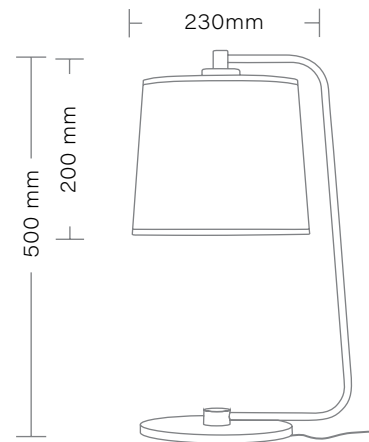
COLUMBUS Lampa gabinetowa/ Big table lamp max 1 x 40W Gwint/Chip: E27 Zasilanie/Power: 230V
