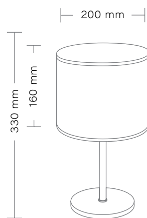
DOS Lampa nocna/ Small table lamp max 1 x 40W Gwint/Chip: E27 Zasilanie/Power: 230V
