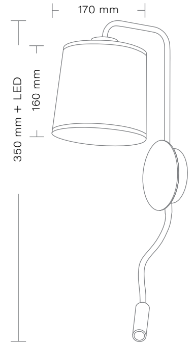
COLUMBUS Kinkiet LED/ Wall lamp LED max 1 x 40W, 1 x 3W LED Gwint/Chip: E27 Zasilanie/Power: 230V
