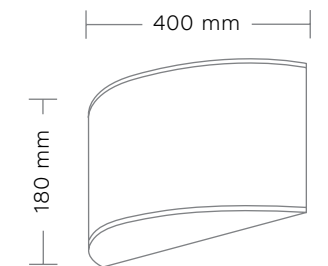
PIANO K-2 Kinkiet/Wall lamp max 2 x 40W, Gwint/Chip: E27 Zasilanie/Power: 230V
