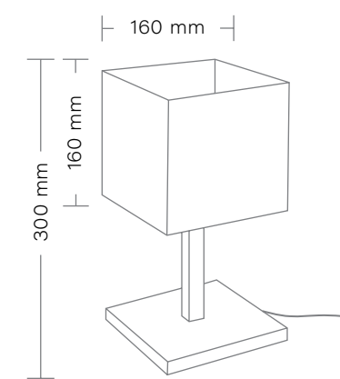
FOBOS Lampa nocna/ Small table lamp max 1 x 40W Gwint/Chip: E27 Zasilanie/Power: 230V
