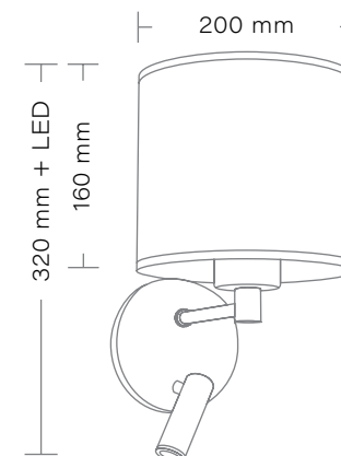
DOS Kinkiet LED / 90 Wall lamp LED / 90 max 1 x 40W 1 x 3W LED Gwint/Chip: E27 Zasilanie/Power: 230V
