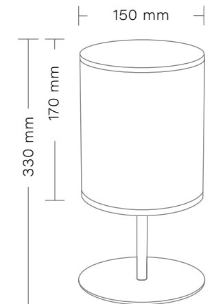
PIANO Lampa nocna/ Small table lamp max 1 x 40W Gwint/Chip: E27 Zasilanie/Power: 230V
