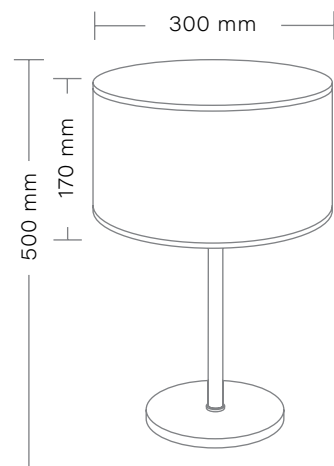
DOS Lampa gabinetowa/ Big table lamp max 1 x 40W Gwint/Chip: E27 Zasilanie/Power: 230V
