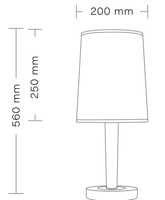
PLATAN Lampa nocna/ Small table lamp max 1 x 40W Gwint/Chip: E27 Zasilanie/Power: 230V
