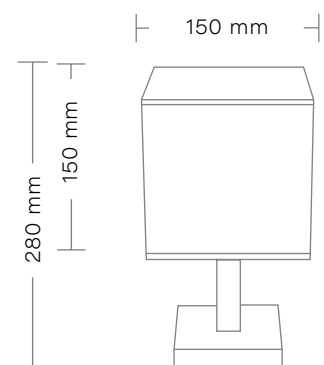
QUATTRO Lampa nocna/ Small table lamp max 1 x 40W Gwint/Chip: E27 Zasilanie/Power: 230V
