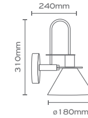
ONNO-WL-B Matt Black Matt Gold E27 Max 40W
