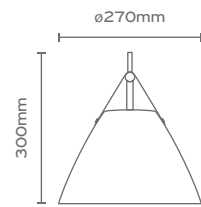
DORIAN S-PL-B Matt Black Black Leather E27 Max 40W
