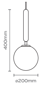
FIORE L-PL Black Opal Glass E27 Max 40W
