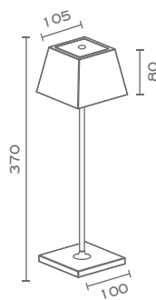
LITTA 2-TL-W White Matt LED 2.2W 231lm 3000K Touch Smooth Dimmer
