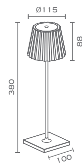
LITTA 1-TL-RU Rust Matt LED 2.2W 231lm 3000K Touch Smooth Dimmer
