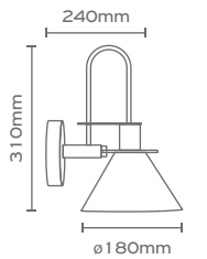
ONNO-WL-W Matt White Matt Gold E27 Max 40W
