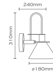
ONNO-WL-G Matt Grey Matt Gold E27 Max 40W
