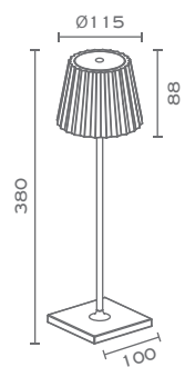
LITTA 1-TL-B Black Matt LED 2.2W 231lm 3000K Touch Smooth Dimmer
